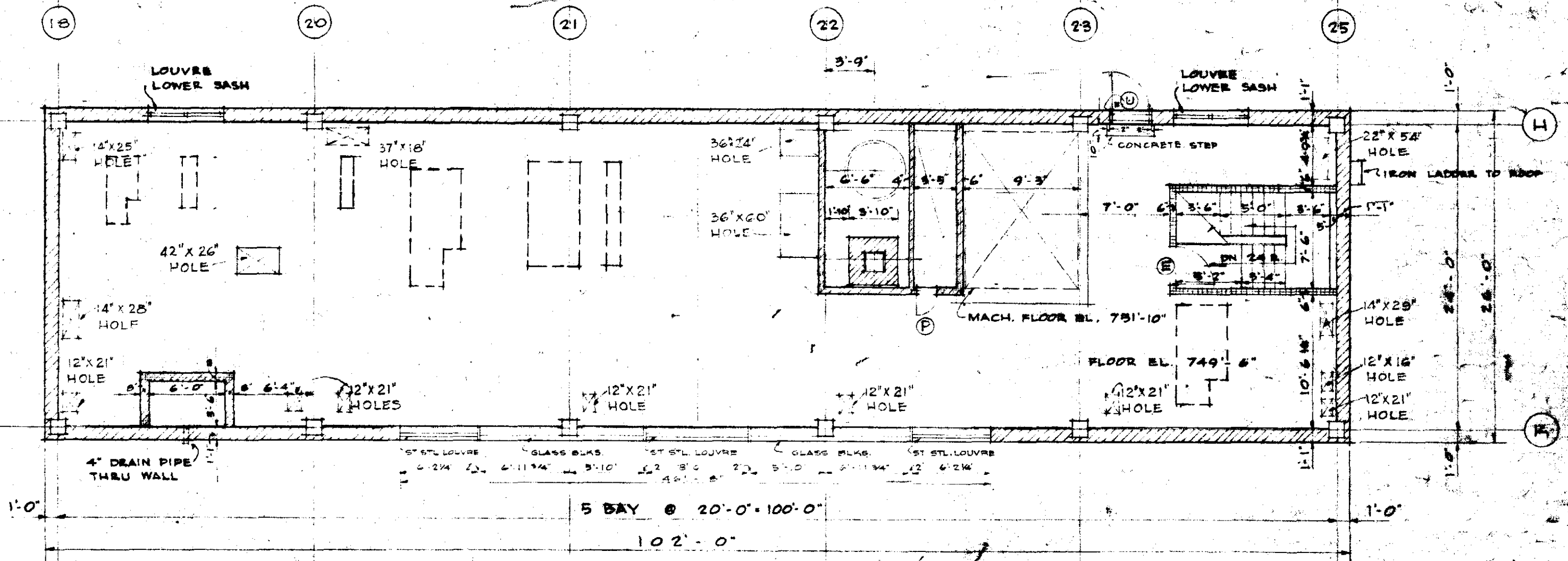
PENT HOUSE FLOOR PLAN SCALE 1/8" = 1'-0"
